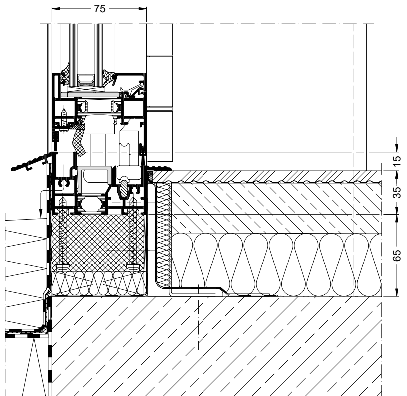
Bottom attachment The Schüco AS FD 75 with 15 mm threshold
